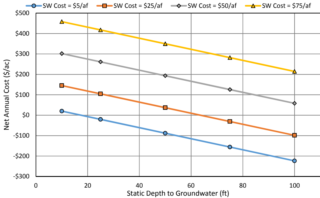
Figure 6-15 Estimated Net Annual Cost of Dual Source System for Example 320-Acre Rice Field with Surface Water Costs of $5/af to $75/af and Static Depth to Groundwater of 10 ft to 100 ft
