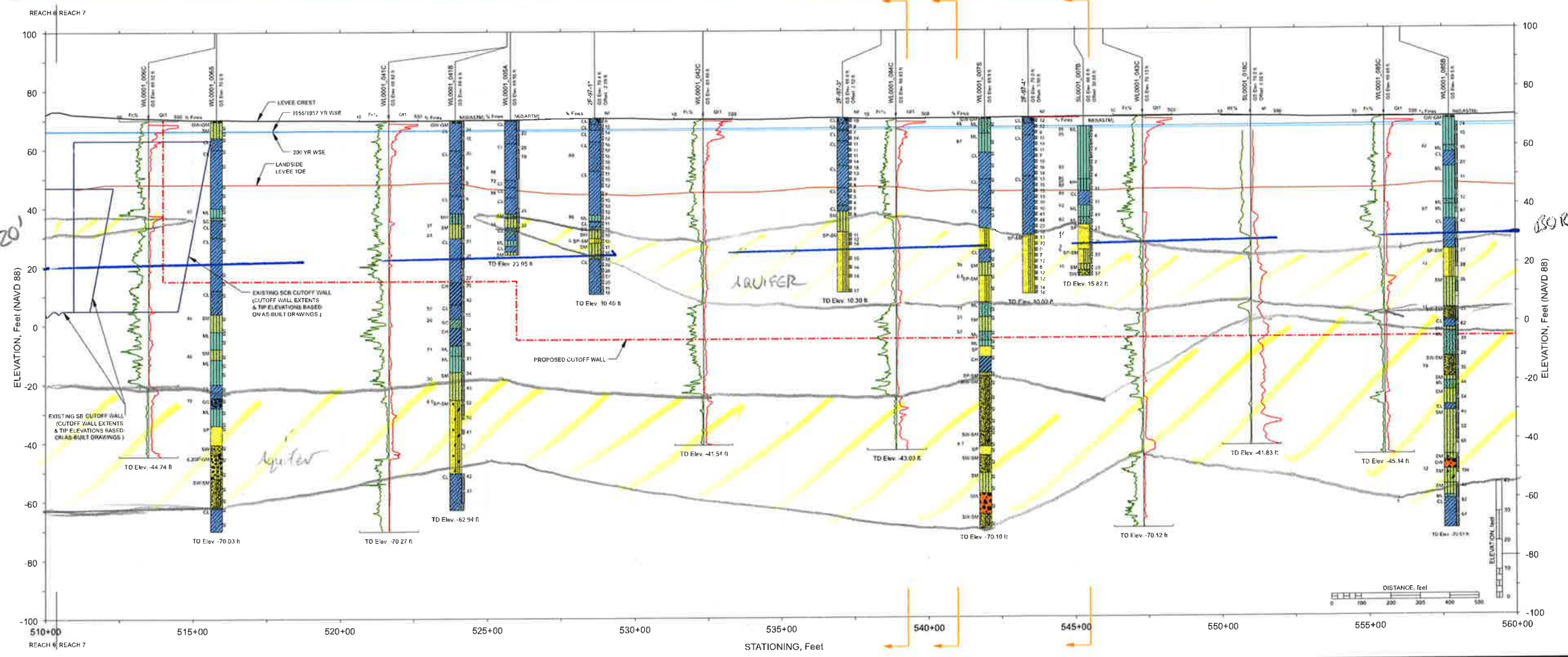
FRWL Project Plan Views and Stick Log Figures FRWL Project: Station 510+00 to Station 560+00
